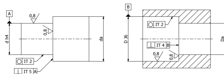
Housing
