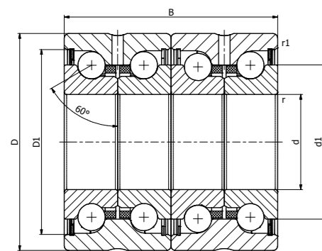
SEL/N...2RS.2AP
