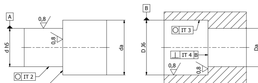
Housing
